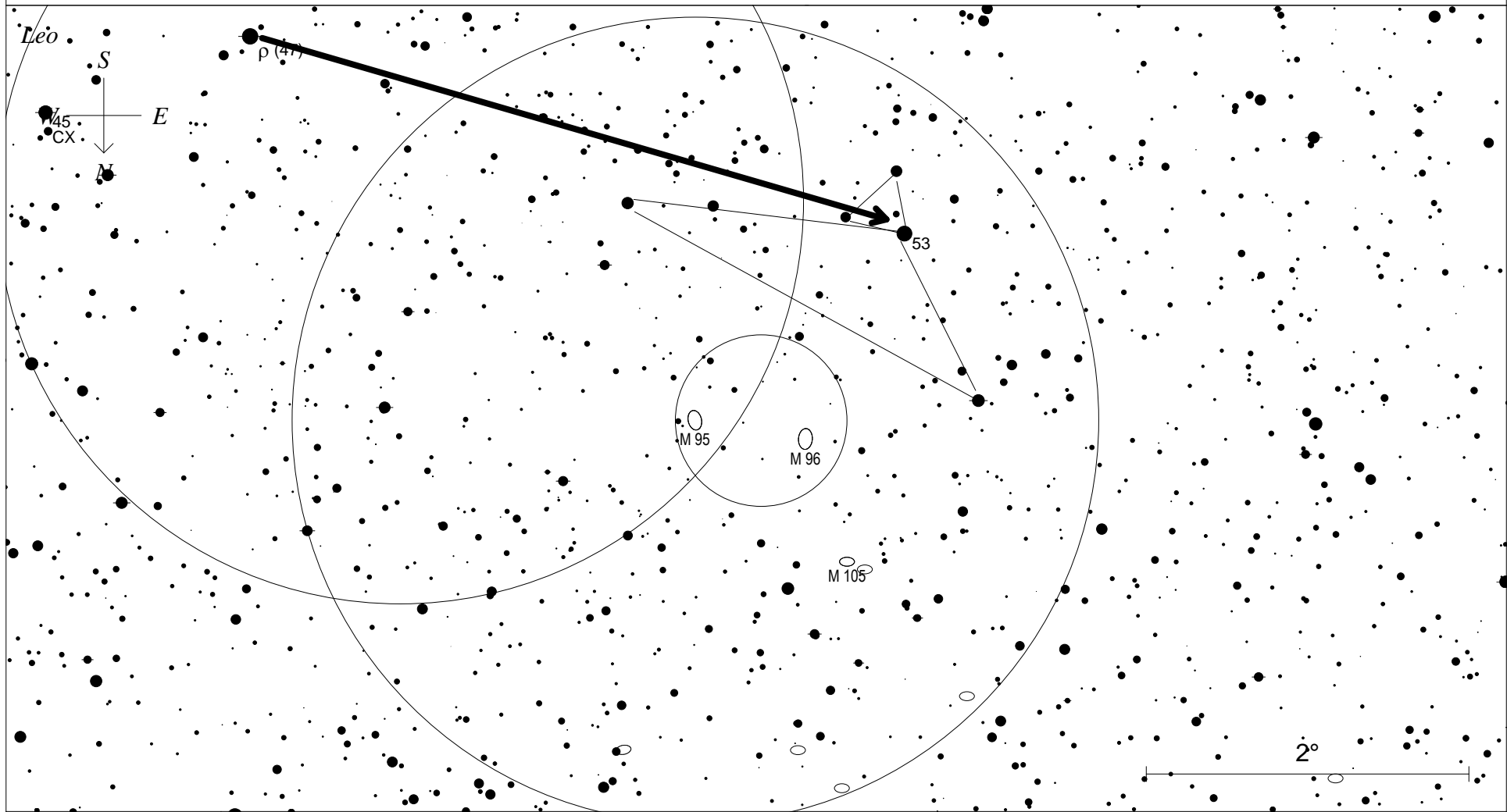
Figure 21 Eyepiece View of M95 95 105
